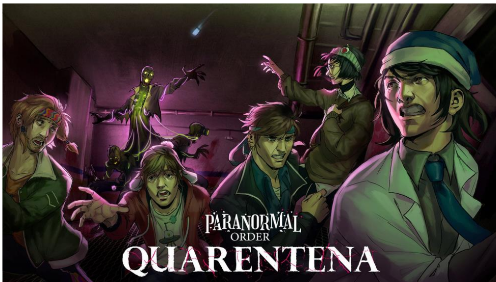
Figura 7 - Especial Two-Shot
